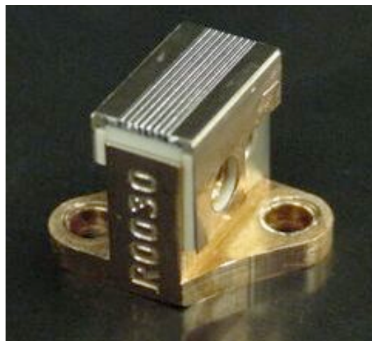
8-Bar Laser Diode Array
